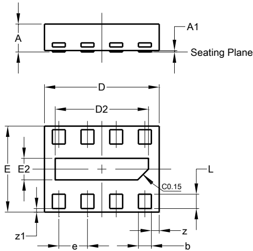
X2-DFN1612-8
