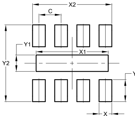
X2-DFN1612-8
