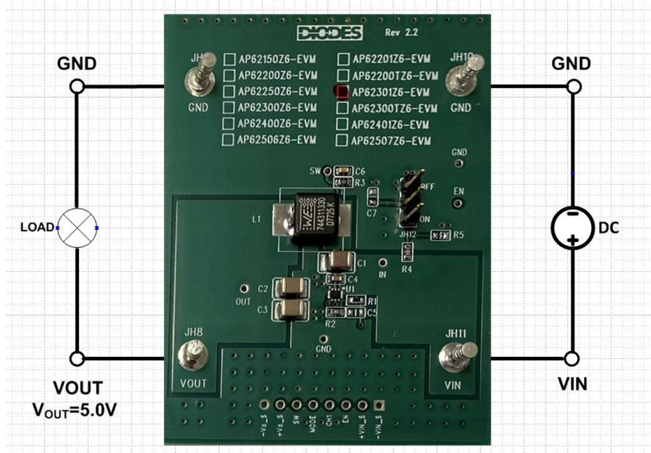
Figure 1. AP62301Z6-EVM
