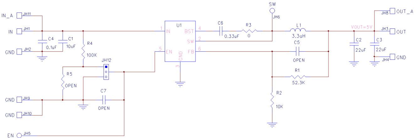
Figure 2. AP62301Z6-EVM Schematic
