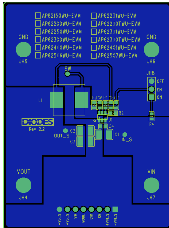
Figure 3. AP62301Z6-EVM – Top Layer
