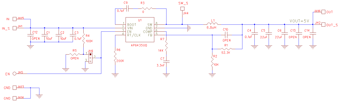
Figure 3. AP64350QSP-EVM Schematic
