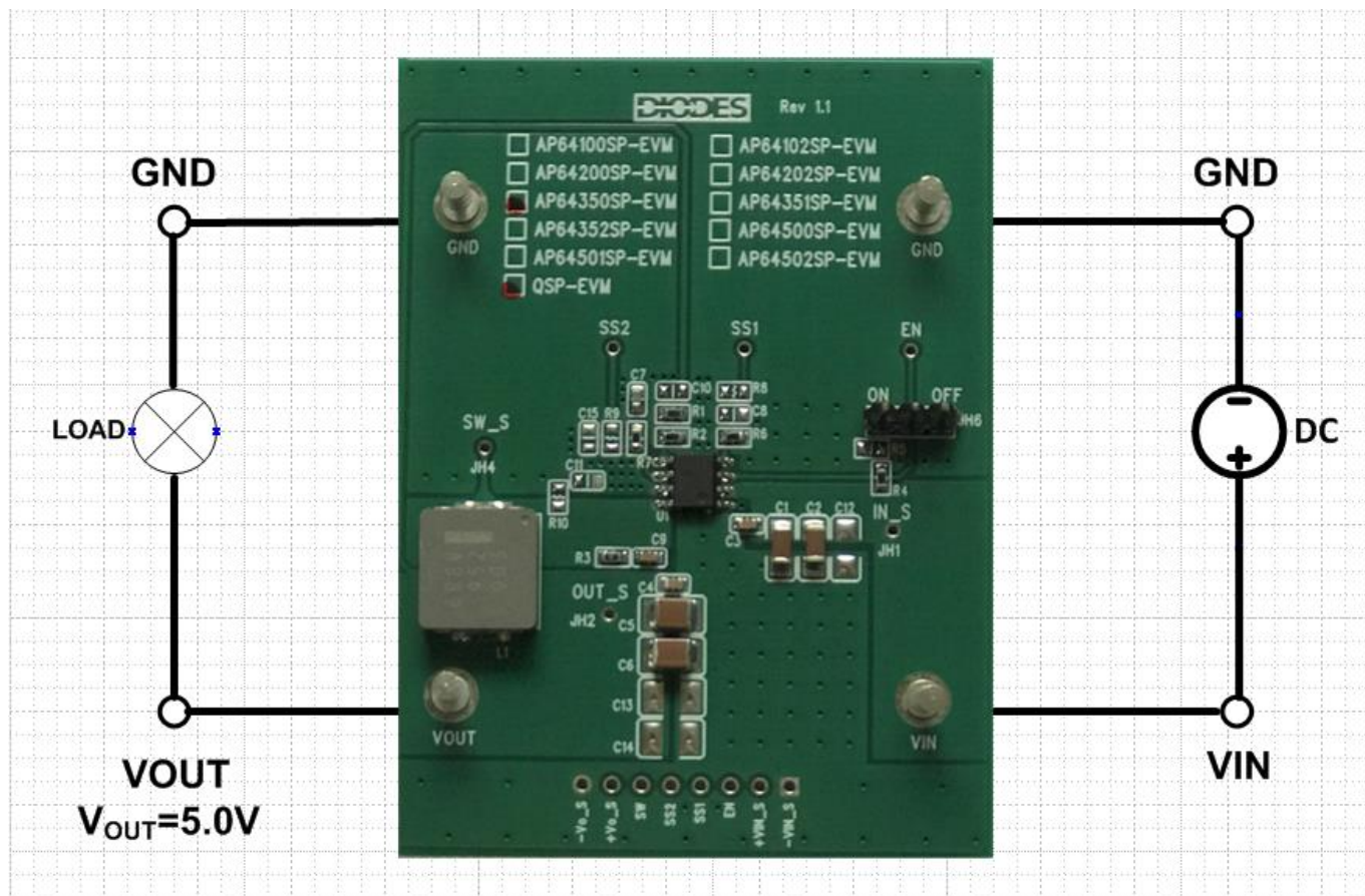
Figure 2. AP64350QSP-EVM
