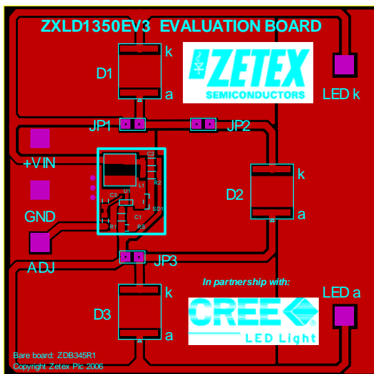
Figure 3: Top View
