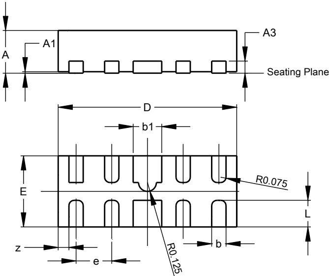
U-DFN2510-10
