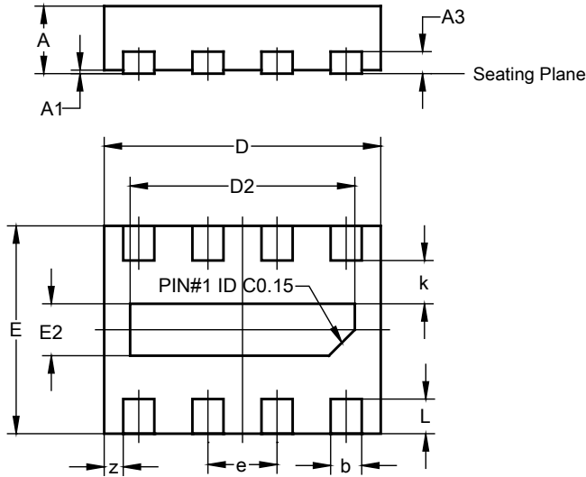
X1-DFN1612-8 (Type B)
