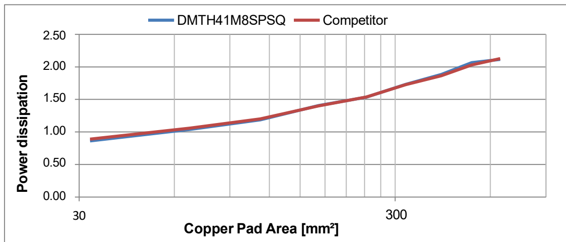
Figure 5. P_D vs. Pad Area—DMTH41M8SPSQ and competitor device
