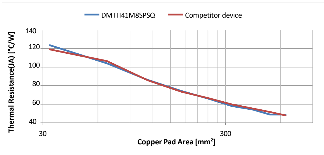
Figure 4. R_{\theta JA} vs. Pad Area—DTMH41M8SPSQ and competitor device
