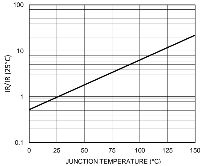
Figure 6. Reverse Leakage Current vs. T_J
