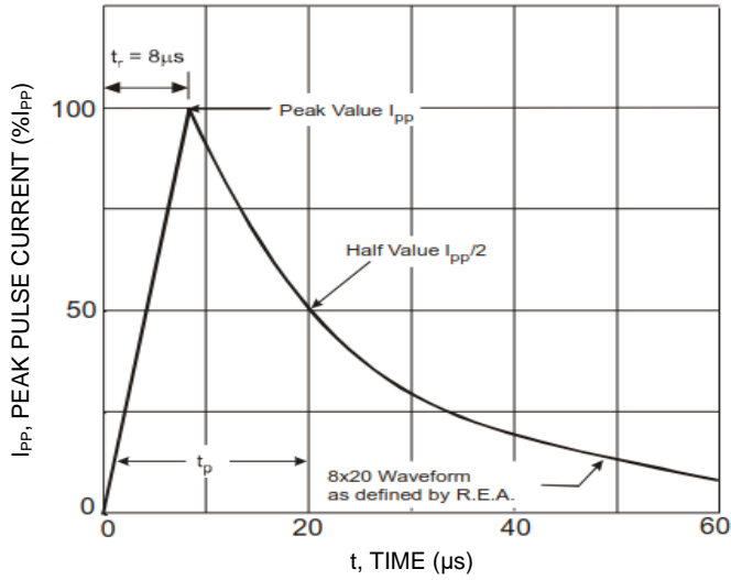
Figure 3. Typical 8 × 20µs Pulse Waveform
