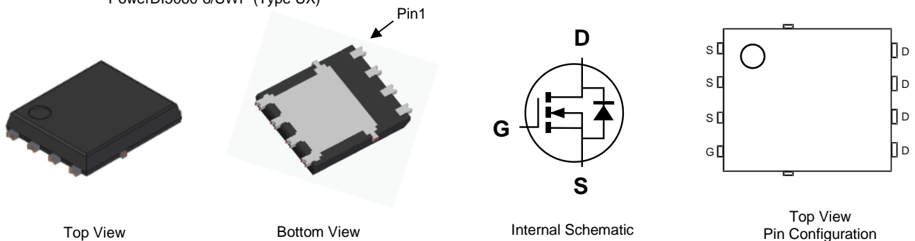
PowerDI5060-8/SWP (Type UX)
