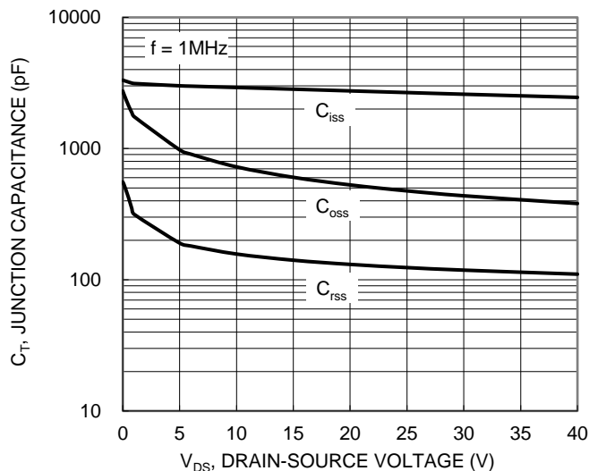
Figure 11. Typical Junction Capacitance
