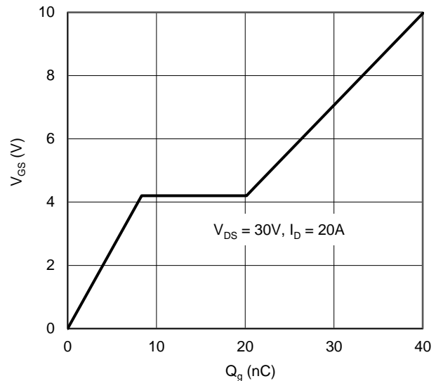
Figure 12. Gate Charge
