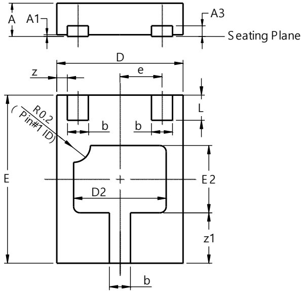
X2-DFN2015-3
