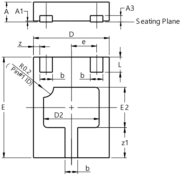
X2-DFN2015-3
