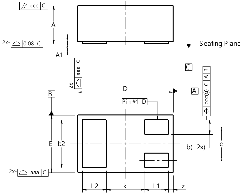
X2-DFN1006-3
