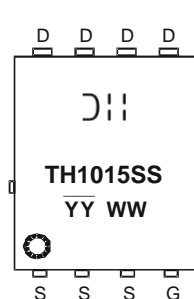
PowerDI5060-8/SWP (Type UX)
