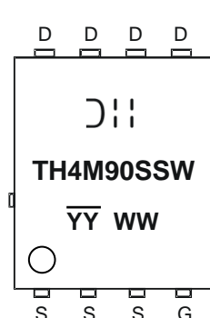
PowerDI5060-8/SWP (Type UX)
