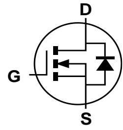
Equivalent Circuit
