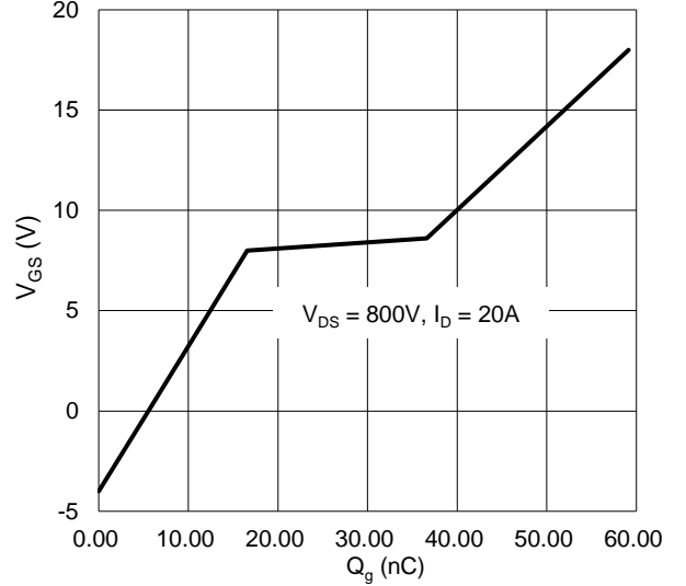
Figure 14. Gate Charge
