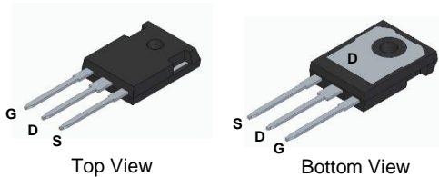
Pin Configuration
