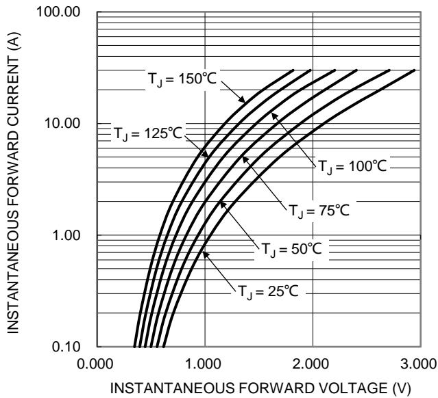
Figure 3. Typical Forward Characteristics
