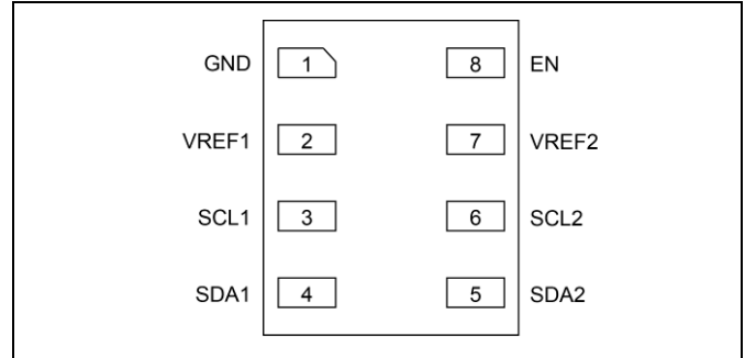
X2-DFN-8(HK)
