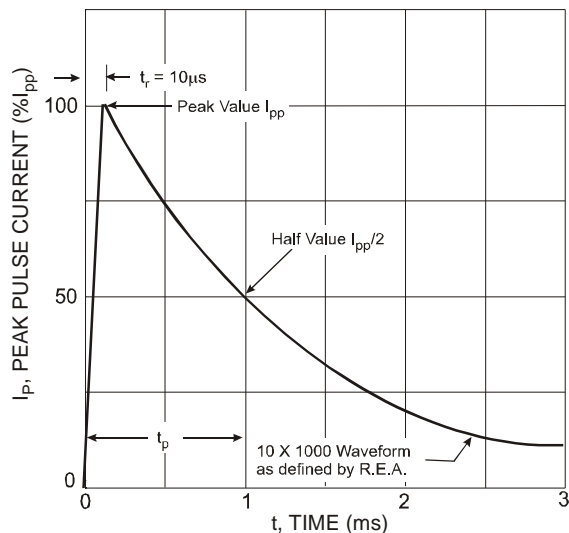
Figure 3 Pulse Waveform
