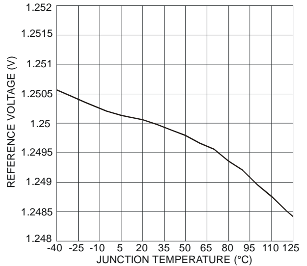
Figure 8 V REF vs. Temperature
