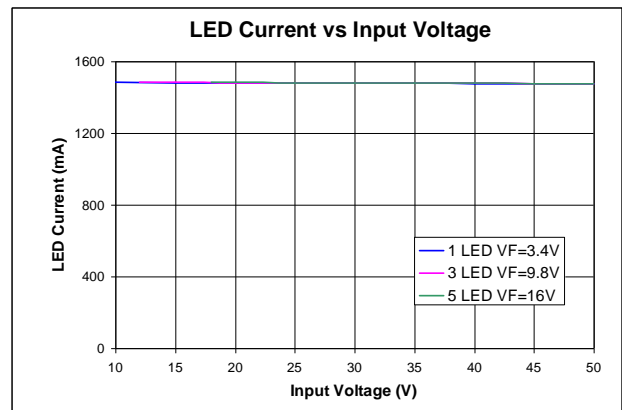
Figure 48 Line Regulation
