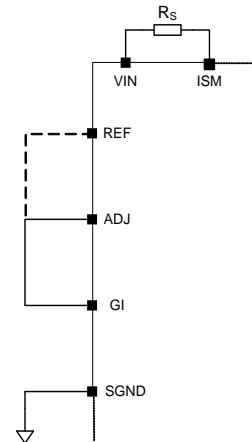
Figure 30 Buck Configuration
