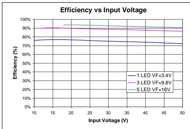
Figure 47 Efficiency
