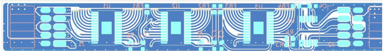
Figure 24. AL58263EV2 PCB Bottom Layer View
