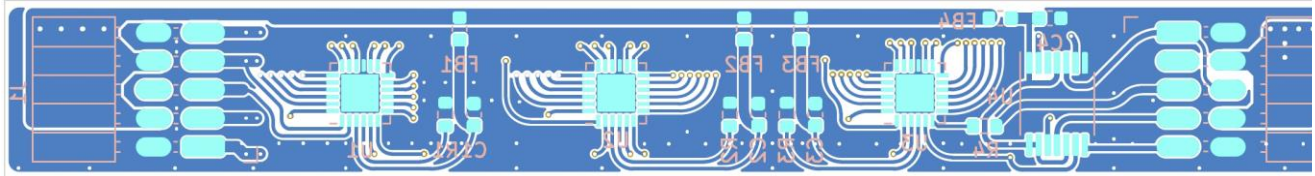
Figure 28. AL58263QEV2 PCB Bottom Layer View
