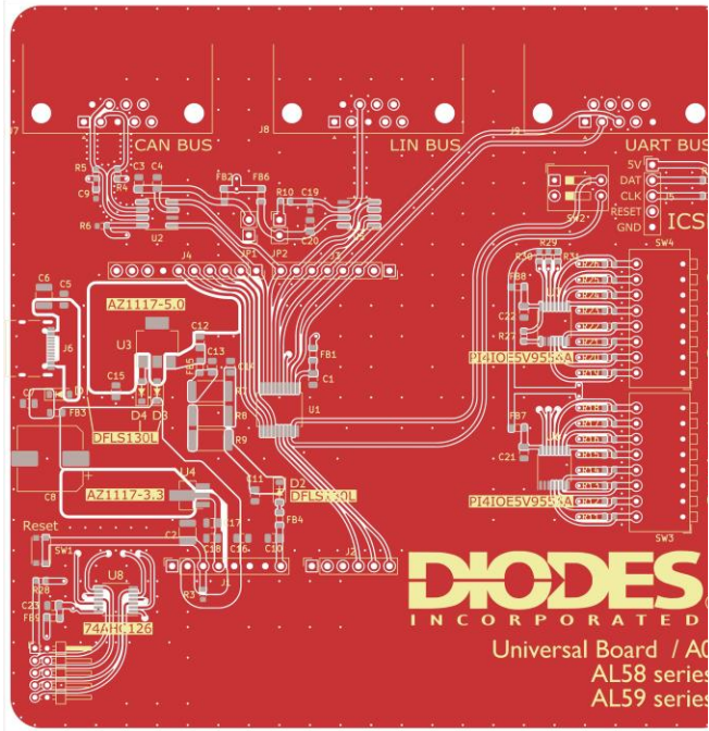
Figure 19. Universal PCB Top Layer View
