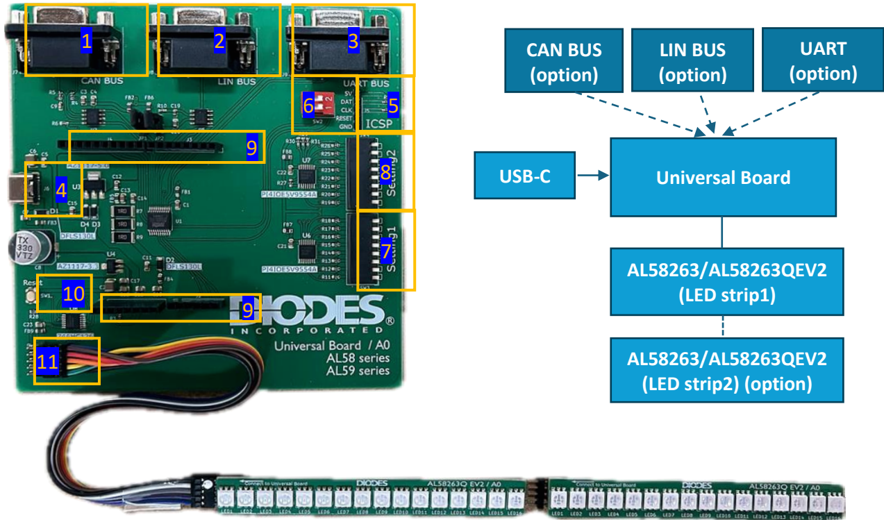
Figure 5. Evaluation Kit Top View
