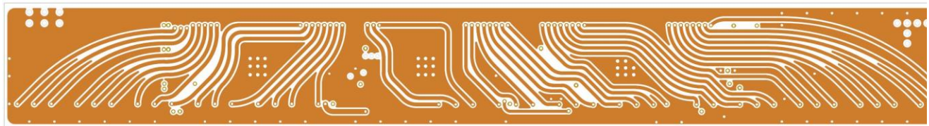
Figure 23. AL58263EV2 PCB Layer2 View
