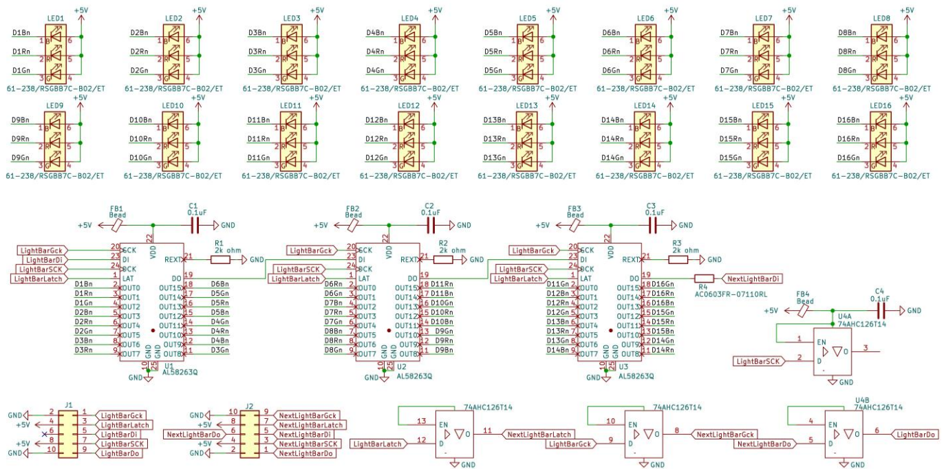
Figure 18. AL58263Q Evaluation Board Schematic
