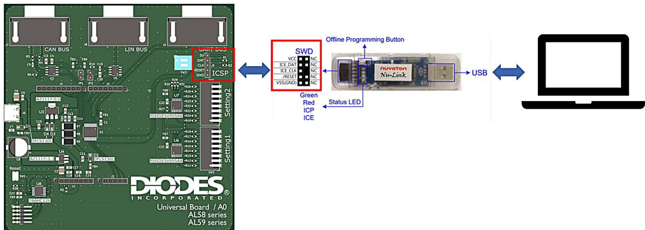
Figure 14. Hardware Connections
