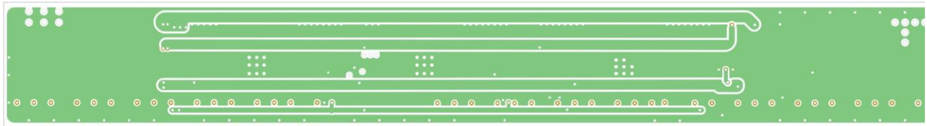
Figure 22. AL58263EV2 PCB Layer1 View
