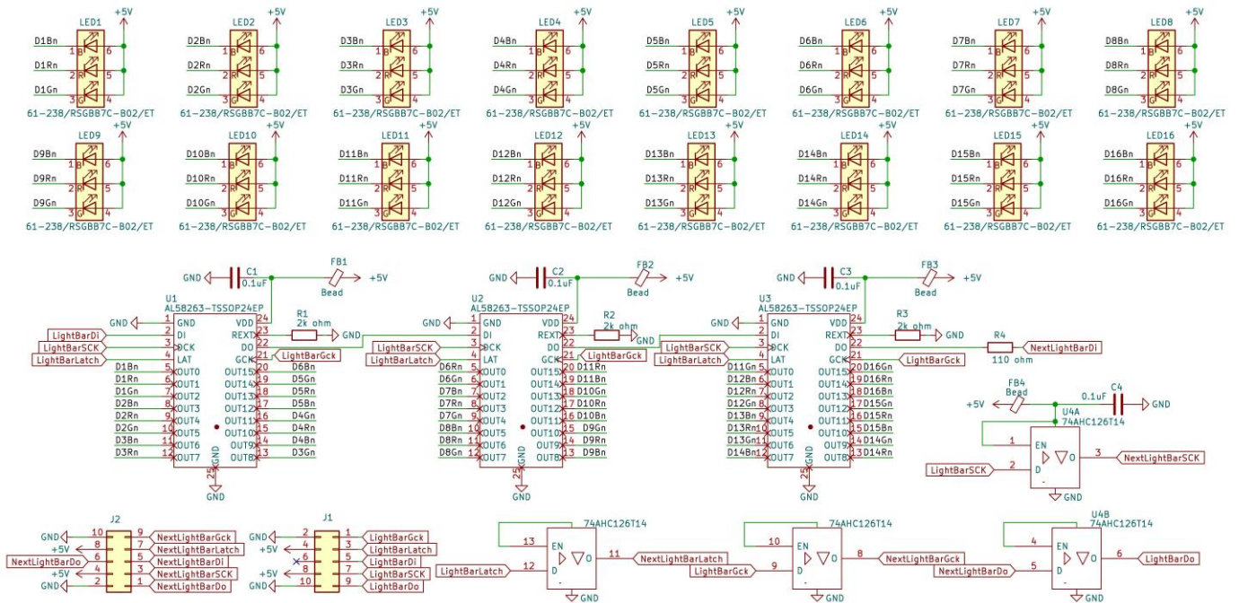
Figure 17. AL58263 Evaluation Board Schematic
