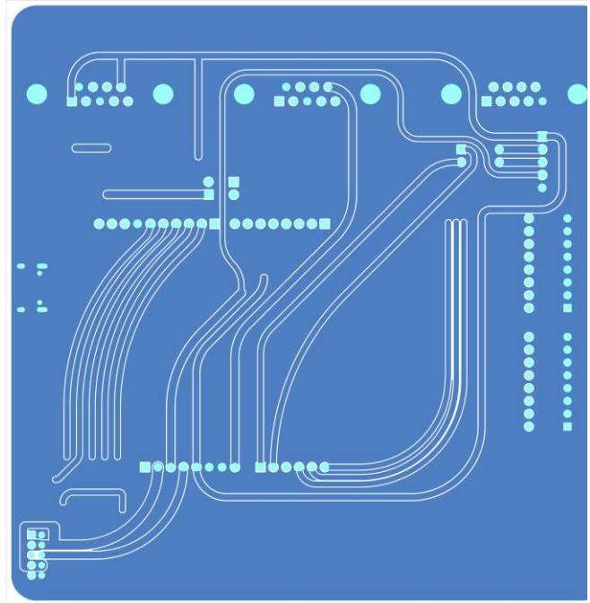
Figure 20. Universal PCB Bottom Layer View
