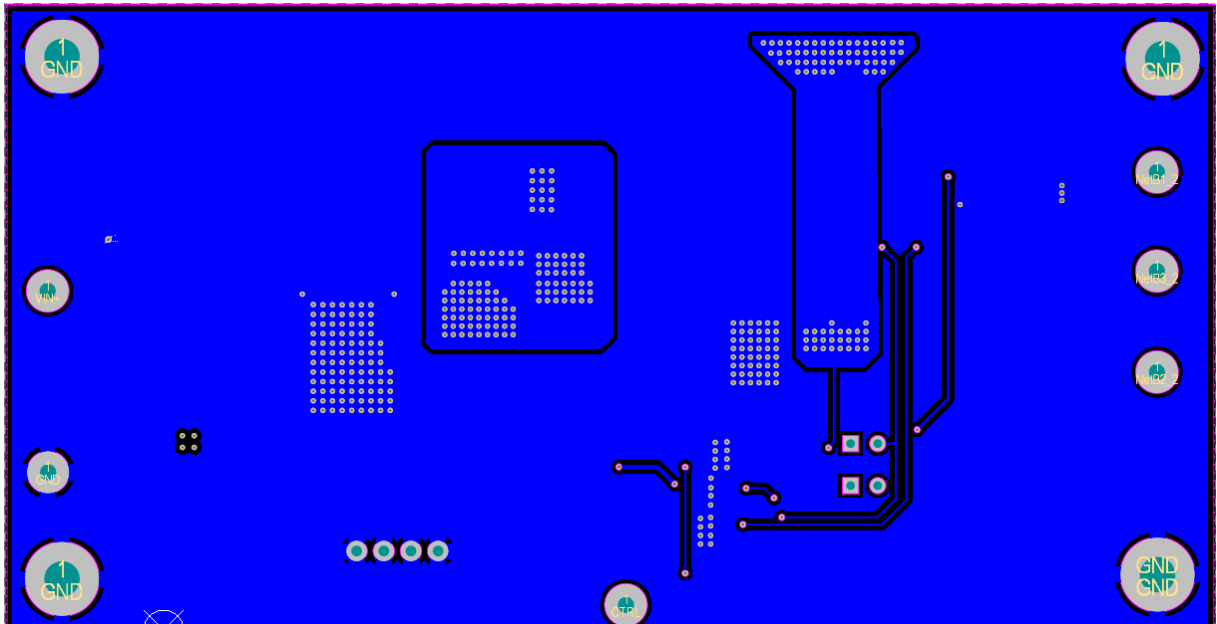
Figure 5: PCB Layout Bottom Layer View
