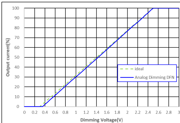
Analog Dimming
