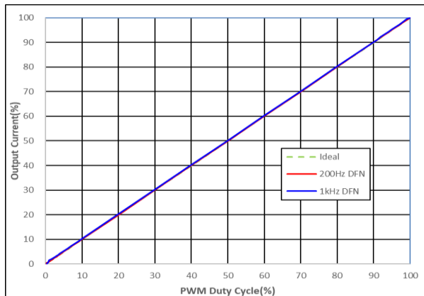
PWM Dimming
