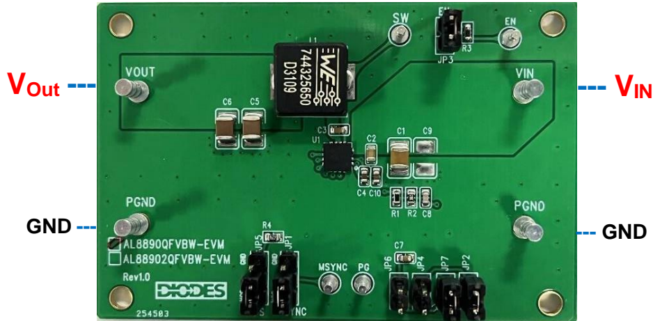
Figure 1: AL8890QFVBW EVM Top View
