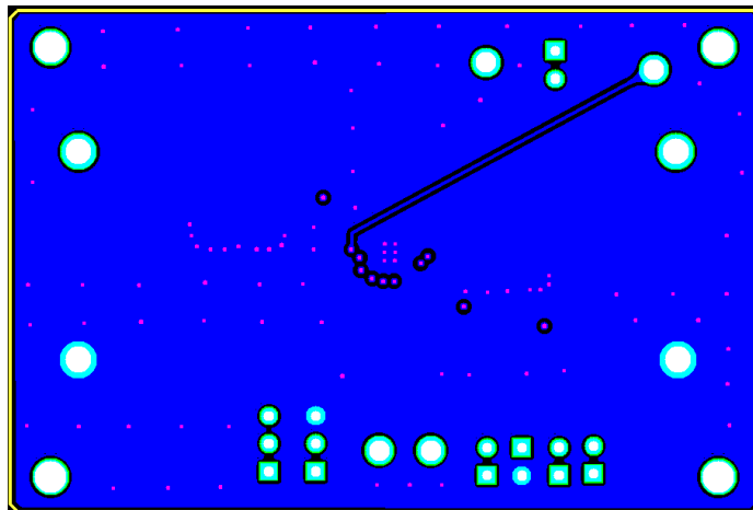
Figure 5: PCB Bottom Layer (Top View)
