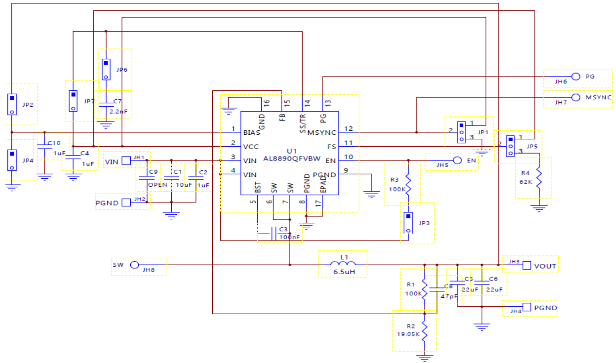
Figure 6: Schematic Circuit
