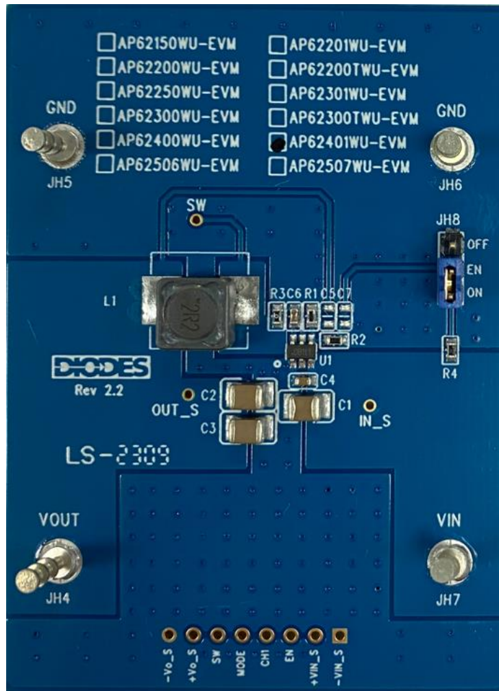
Figure 1. AP62401WU-EVM
