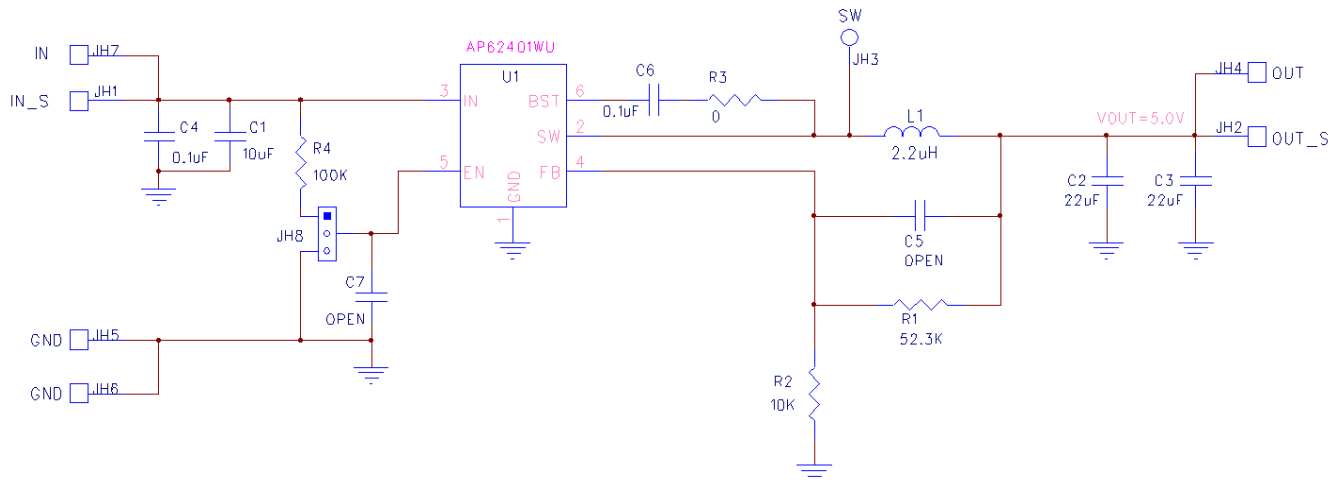
Figure 2. AP62401WU-EVM Schematic
