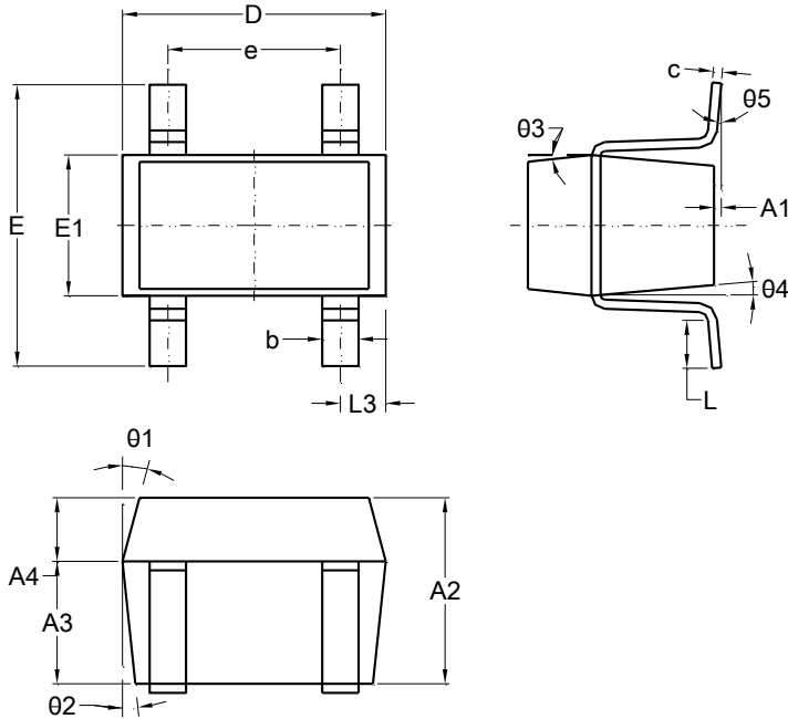
SOT23-4 (Type B)
