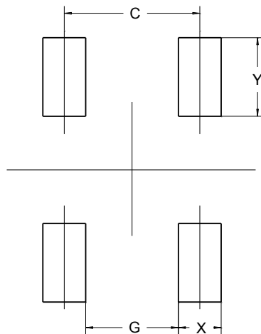
SOT23-4 (Type B)
