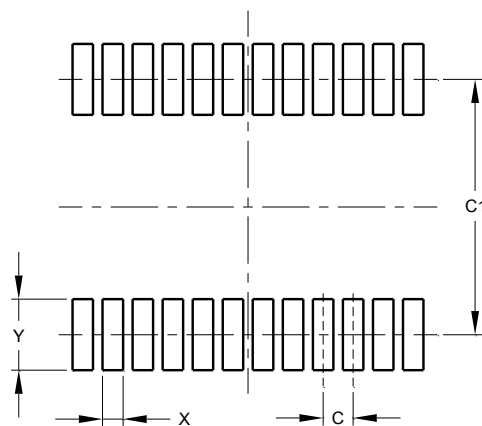
SSOP-24 (Type A1)
