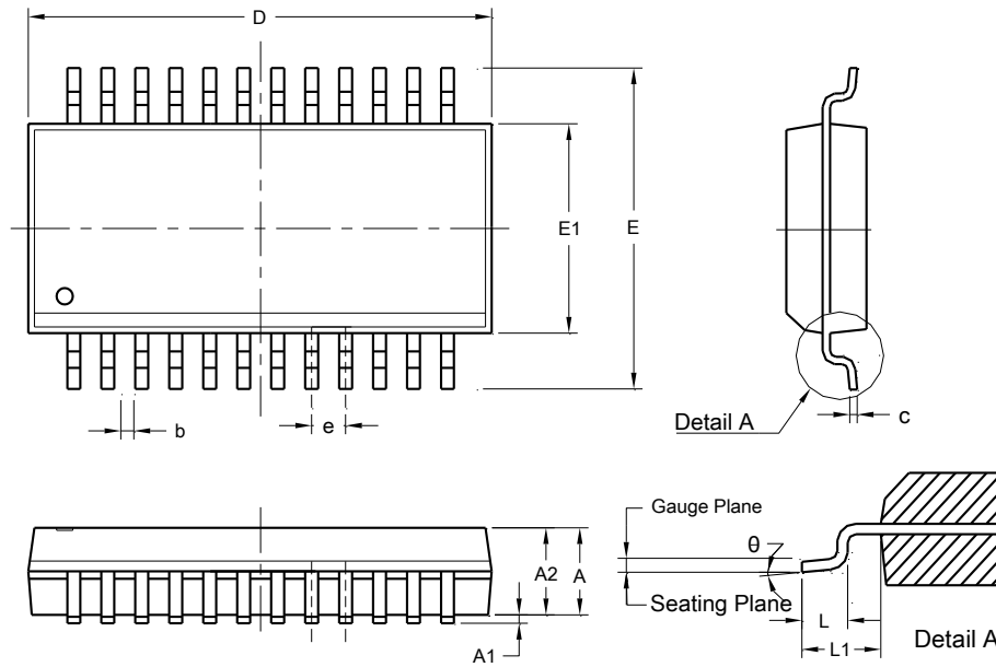
SSOP-24 (Type A1)
