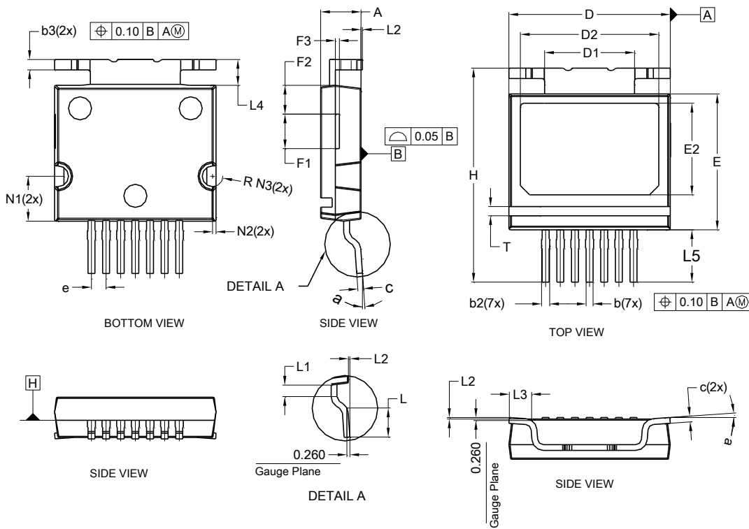
TO263-7 (Type C)
