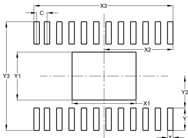
TSSOP-28EP (Type TH-2)
