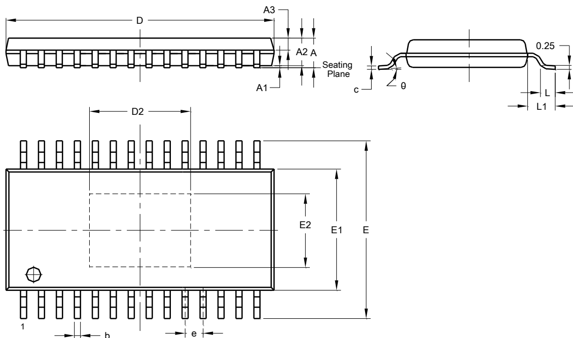
TSSOP-28EP (Type TH-2)
