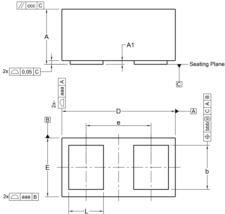
X3-DFN0603-2 (Type E)
