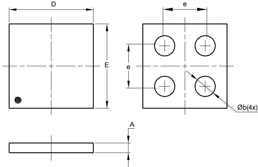
X4-DSN1010-4
