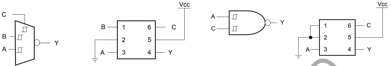
Configuration 2 2-Input NAND Gate 2-Input OR Gate with Both Inputs Inverted
