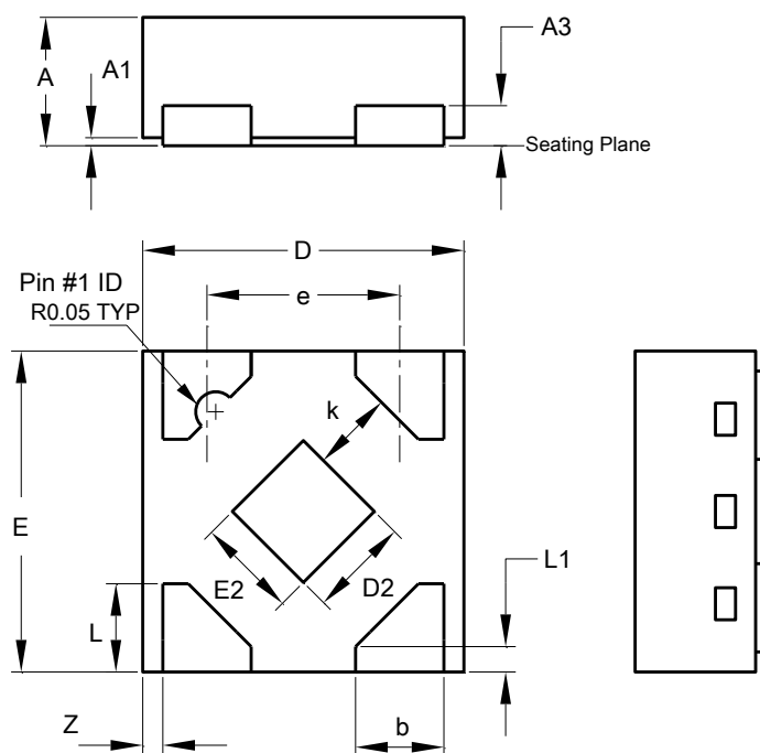
X2-DFN0808-4
