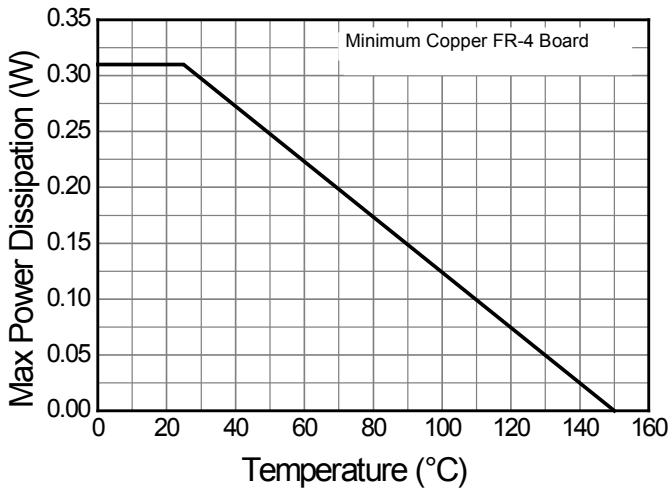
Derating Curve
