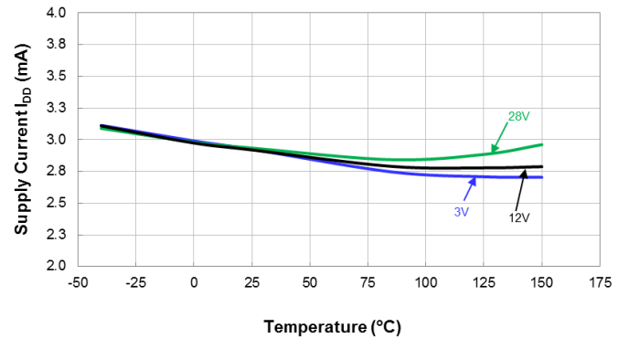
Supply Current vs Temperature
