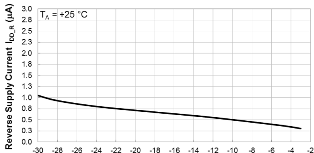
Reverse Supply Current vs Supply Voltage
