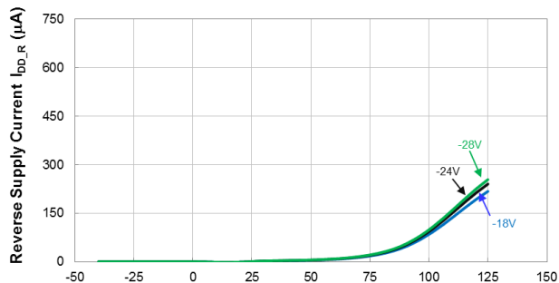
Reverse Supply Current vs Temperature
