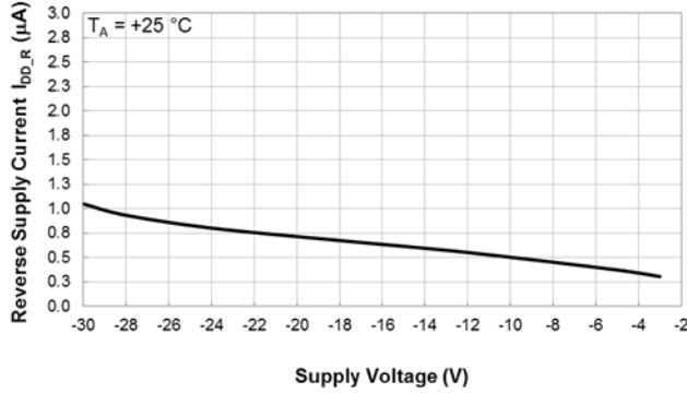
Reverse Supply Current vs Supply Voltage
