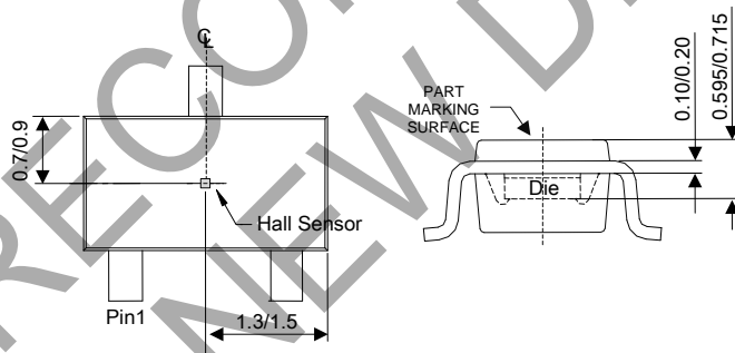
Sensor Location
