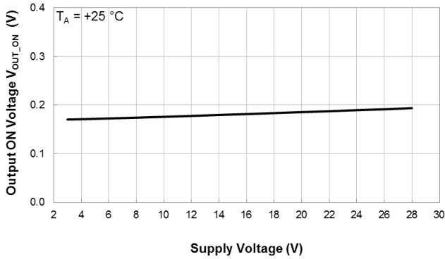
Output ON Voltage vs Supply Voltage
