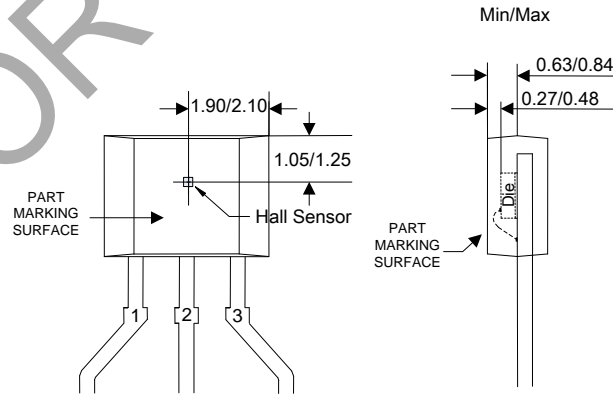
Sensor Location
