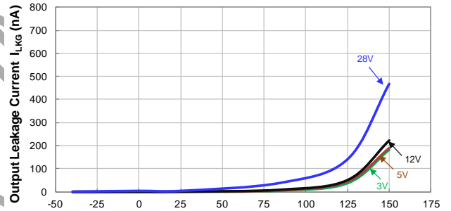
Temperature (°C) Output Leakage Current vs Temperature
