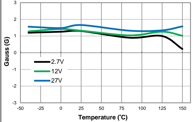
B MATCH (SP B RP - DIR B RP ) vs. Temperature
