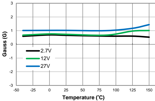
SP B OFF (B OP + B RP )/2 vs. Temperature
