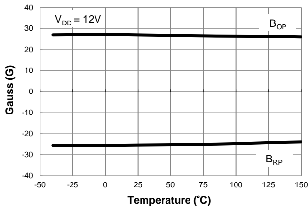
Switch Points vs. Temperature
