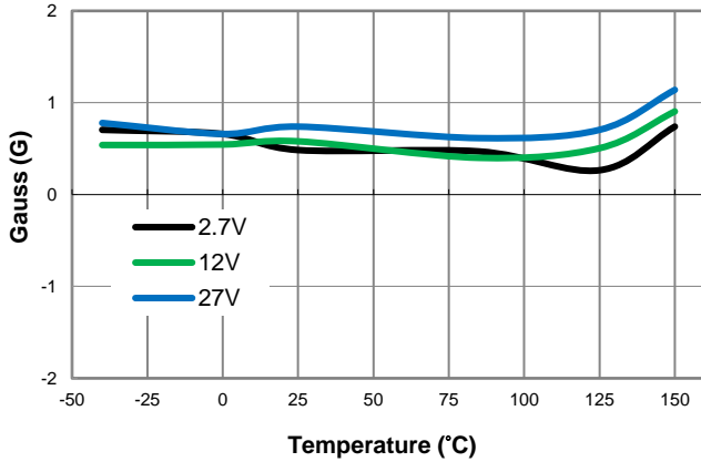
SP B OFF (B OP +B RP )/2 vs. Temperature
