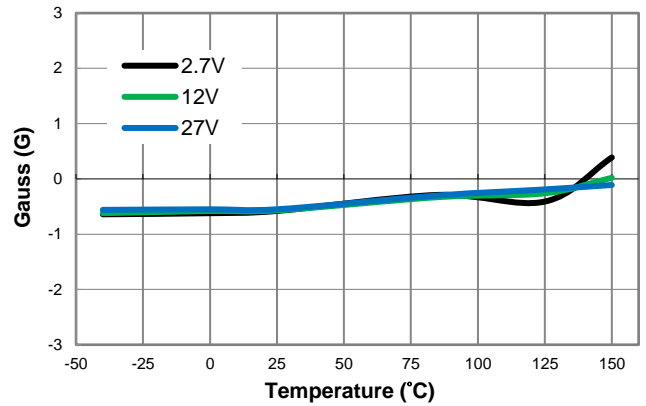
DIR B OFF (B OP + B RP )/2 vs. Temperature
