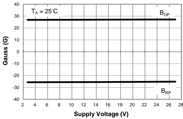
Switch Points vs. Supply Voltage
