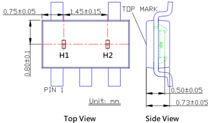
Sensor Location
