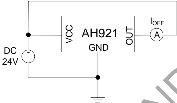
Figure 7. Test Condition of AH921 (Output Leakage Current)
