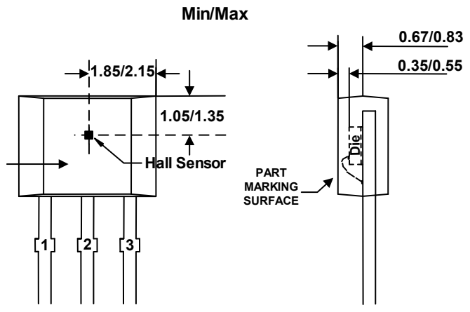
Sensor Location
