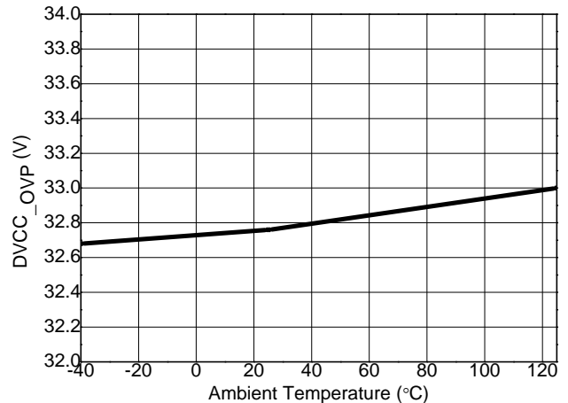
DVCC OVP Voltage vs. Ambient Temperature
