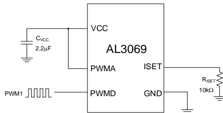
Direct PWM Dimming Operation
