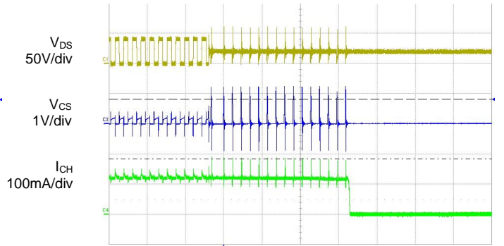
Time: 10 \mu\text{s}/\text{div}
