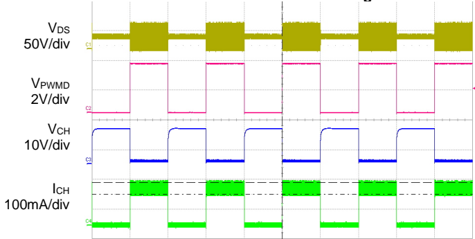
Direct PWM Dimming
