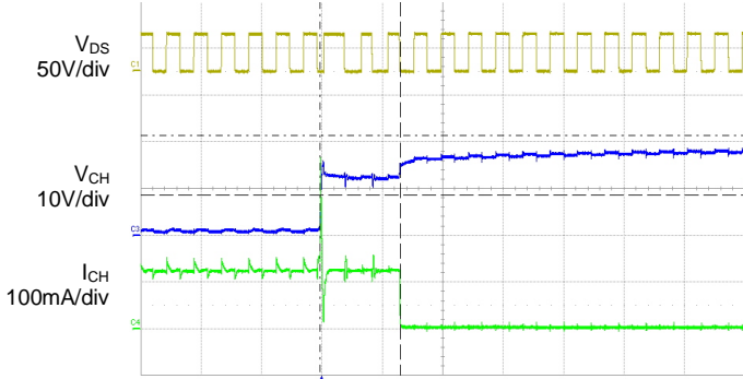
Time: 5 \mu\text{s}/\text{div}
