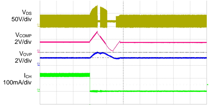
Time: 5ms/div
