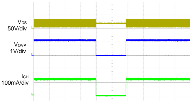
Time: 200ms/div
