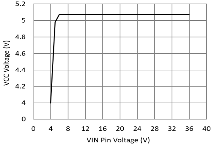
VCC Voltage vs. VIN Pin Voltage
