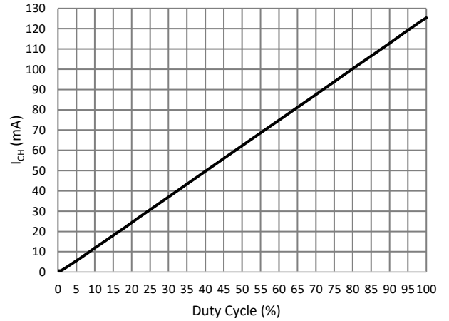
PWM to Analog Dimming Curve @ f_{PWMA} = 100\text{kHz} Channel Current vs. Duty Cycle
