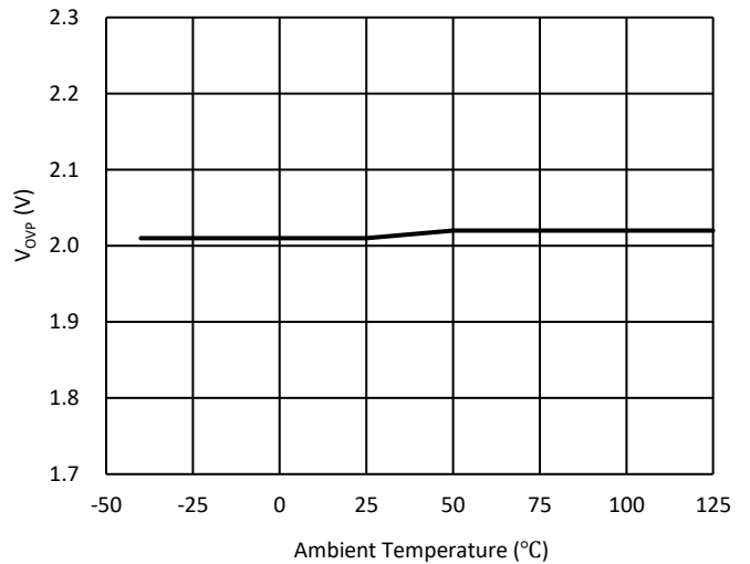
VovP vs. Ambient Temperature
