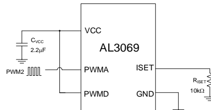
PWM to Analog Dimming Control
