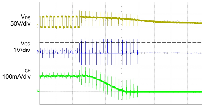
Time: 10 \mu\text{s}/\text{div}
