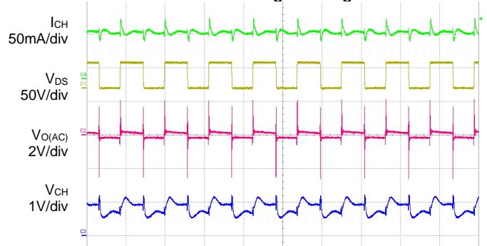
PWM to Analog Dimming
