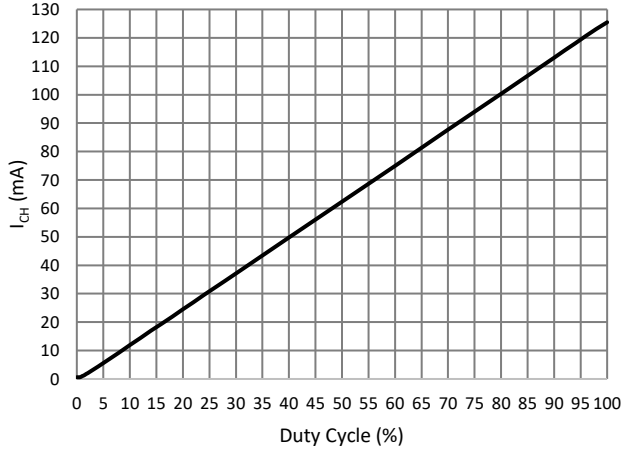
PWM to Analog Dimming Curve @ f_{PWMA} = 5\text{kHz} Channel Current vs. Duty Cycle
