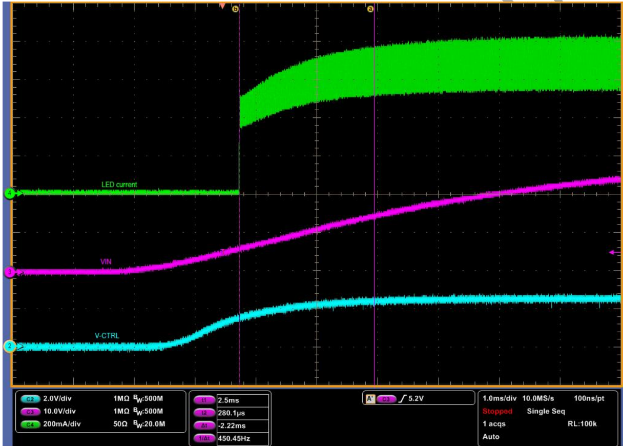
Figure 33 Soft start with 22nF capacitor on CTRL pin ( V_{IN} = 30\text{V} , I_{LED} = 667\text{mA} , 1 LED)
