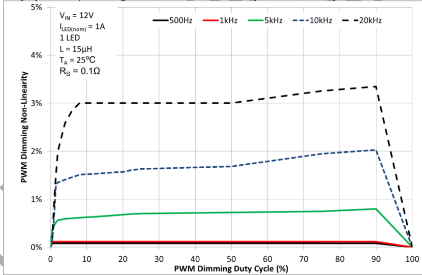
Figure 36 PWM Dimming Non-Linearity at 530kHz nominal switching frequency
