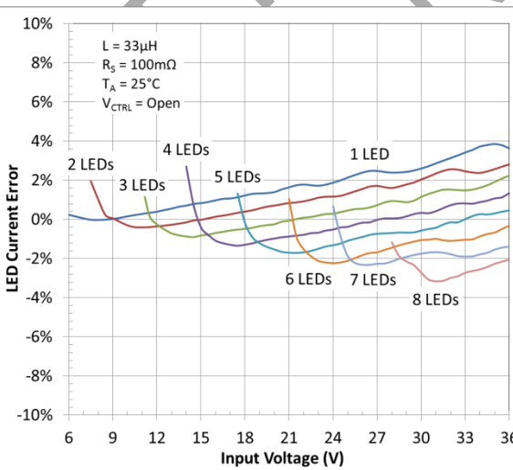
Figure 23. LED Current Deviation vs. Input Voltage
