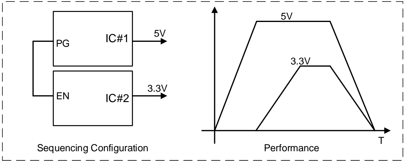
Figure 52. Sequencing Configuration
