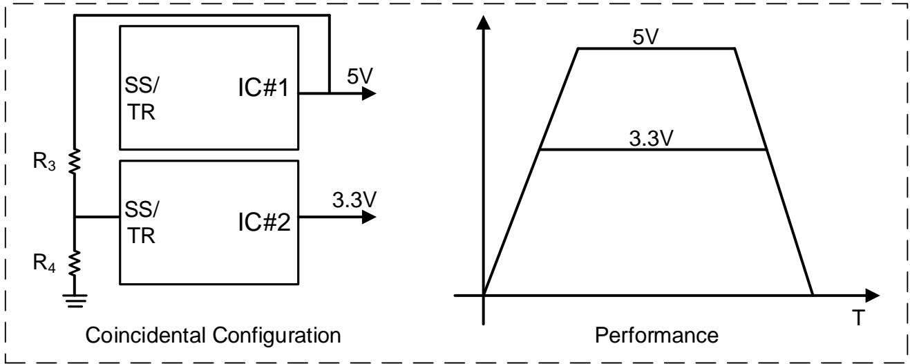
Figure 51. Coincidental Configuration
