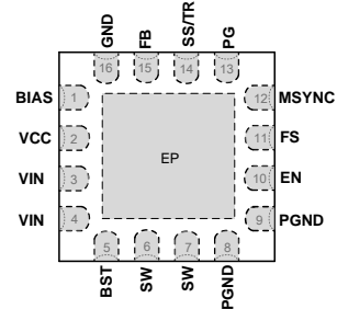
U-QFN4040-16/SWP (Type UXB) (Top View)
