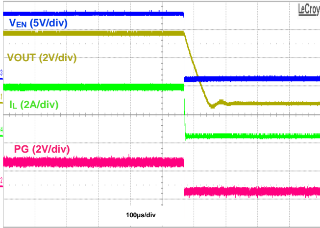
Figure 46. Shutdown using EN with PG, IOU = 3.5A
