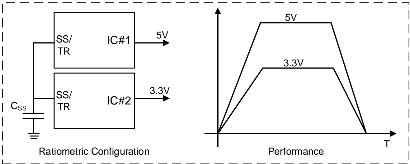
Figure 50. Ratiometric Configuration
