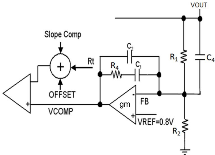
Figure 59. Type 2 Compensator
