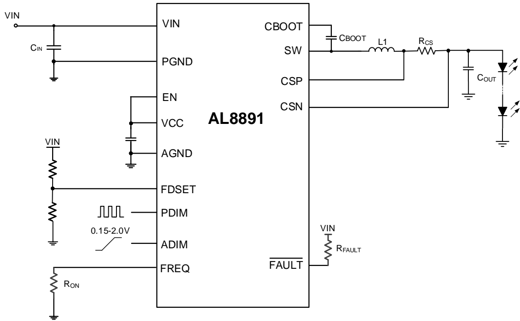
Figure 1. Typical Application
