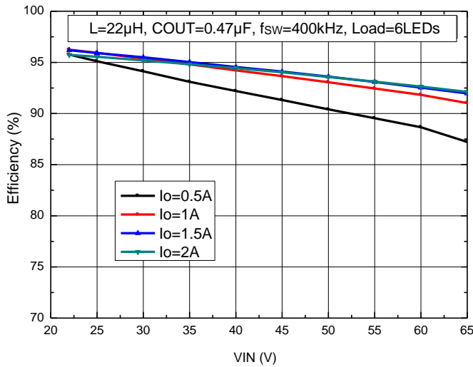
Figure 11. Efficiency vs. VIN
