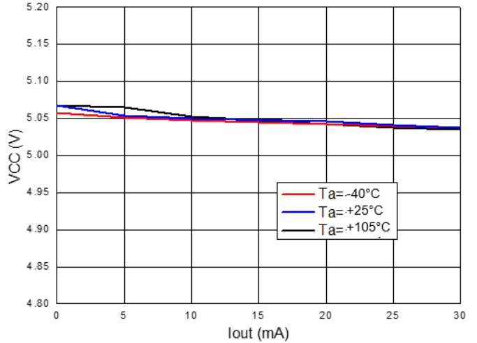
Figure 24. VCC vs. Iout
