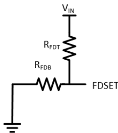
Figure 41. Set VIN Threshold to Mask LED Open Fault
