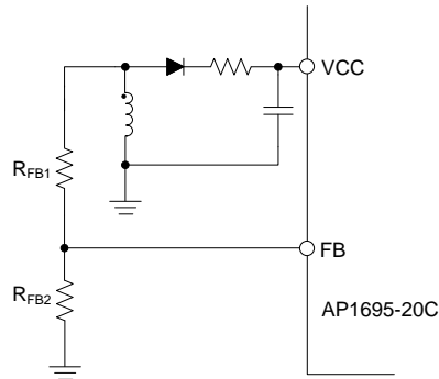
Figure 4. OVP Circuit
